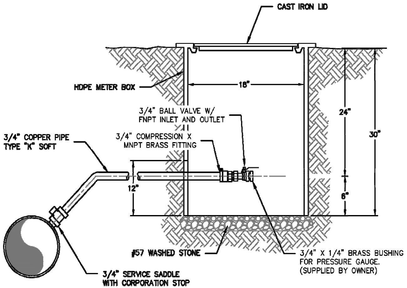
SECTION VIEW
